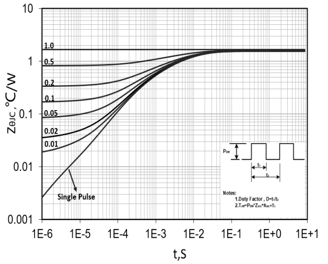
Figure 14. Transient Thermal Response Curve (TO-252/TO-251)
