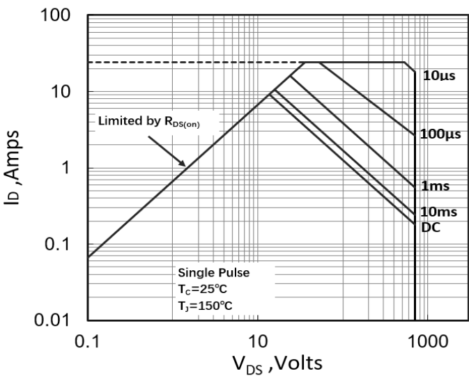
Figure 11. Maximum Safe Operating Area (TO-263/TO-220)
