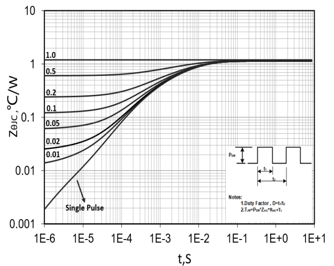
Figure 12. Transient Thermal Response Curve (TO-263/TO-220)
