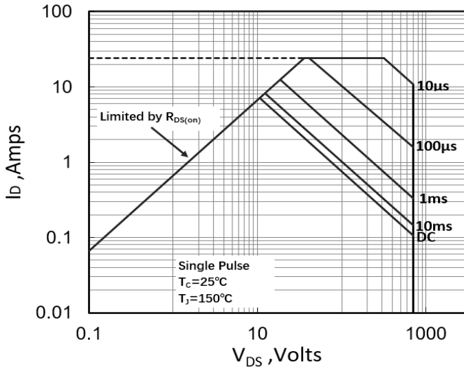
Figure 13. Maximum Safe Operating Area (TO-252/TO-251)
